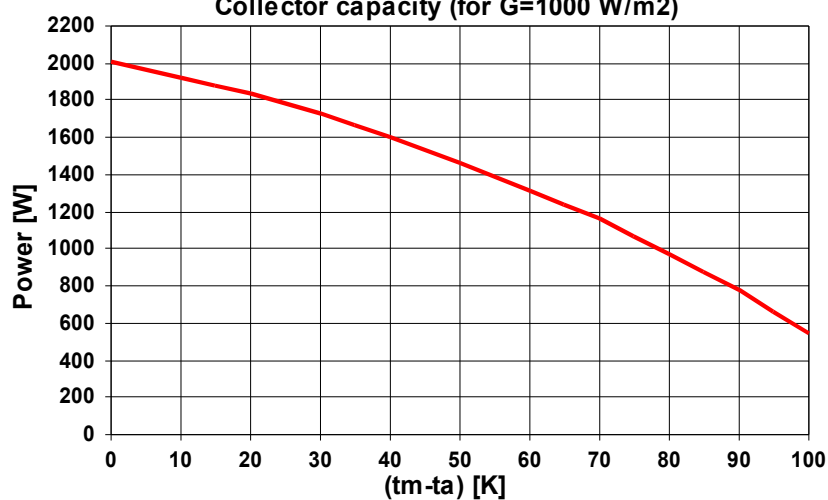
Collector capacity (for G=1000 \text{ W/m}^2 )
