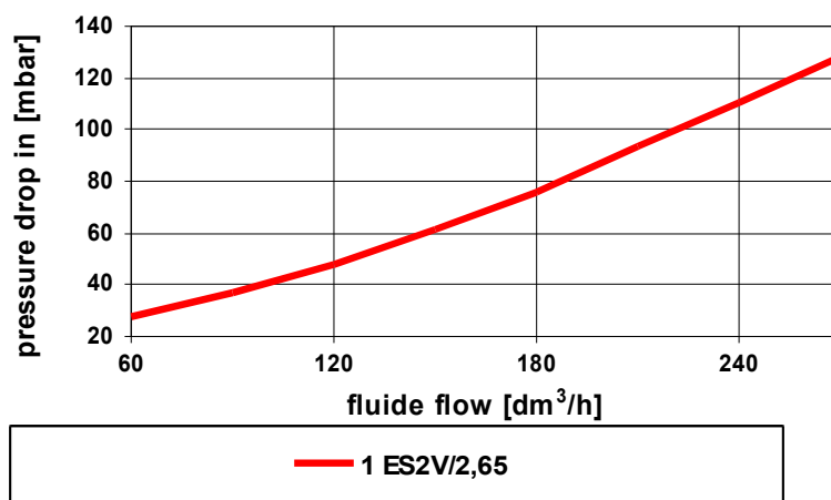
Pressure loss by flow through 1 meander panels ES2V/2,65
